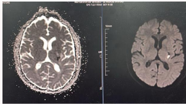
Diffüzyon MR
